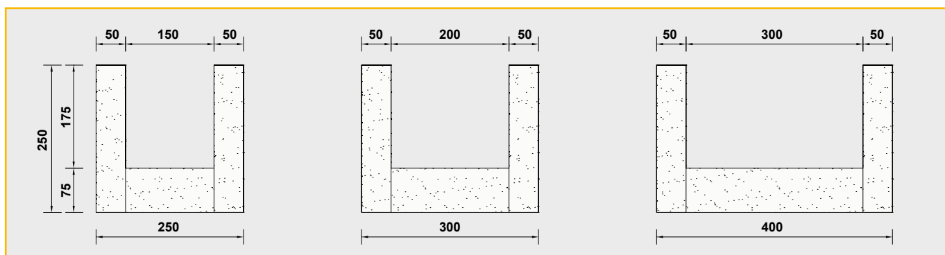
Abmessungen U-Steine (in mm)
